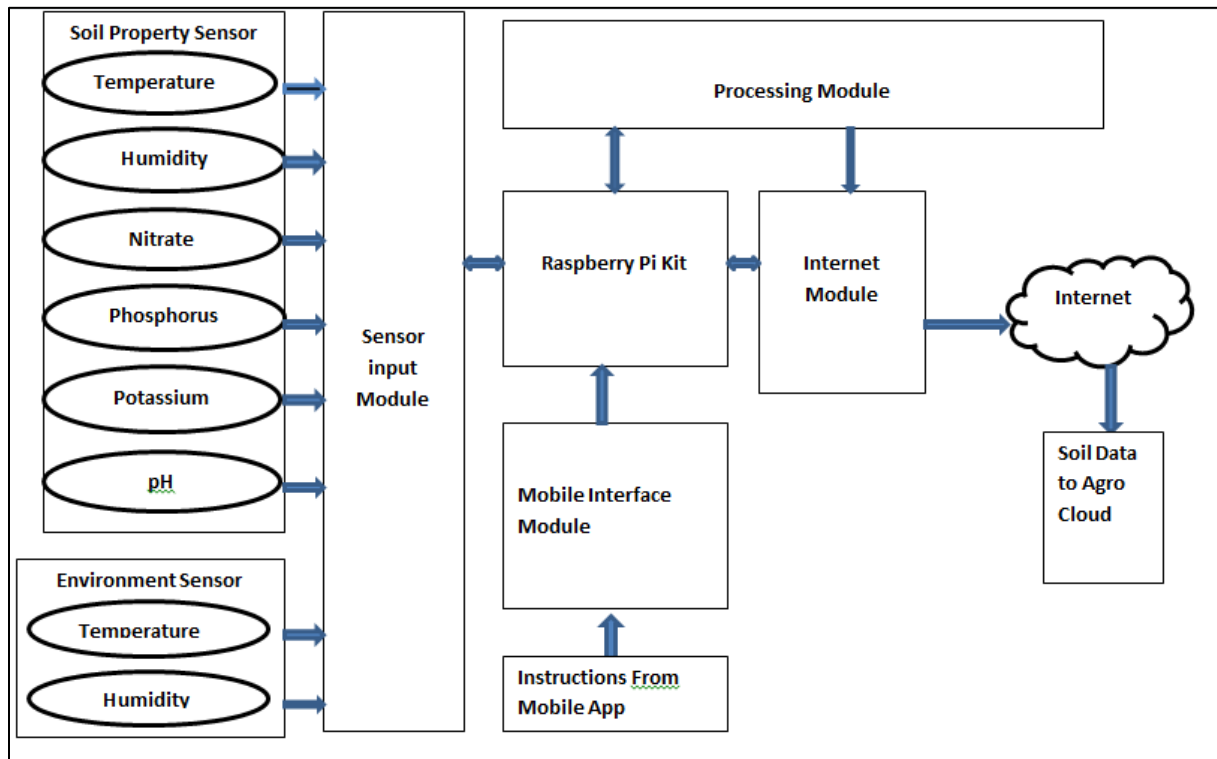
Figure 5: Sensor Kit Module
