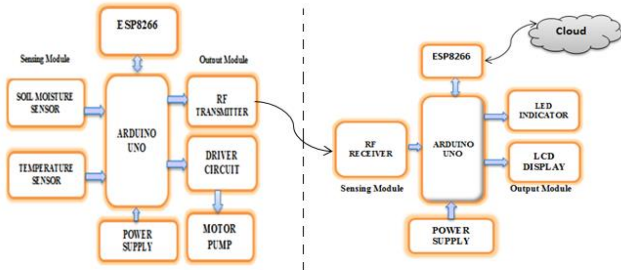
Fig (a).Block Diagram for Transmitter Section Fig (b).Block Diagram for Receiver Section
