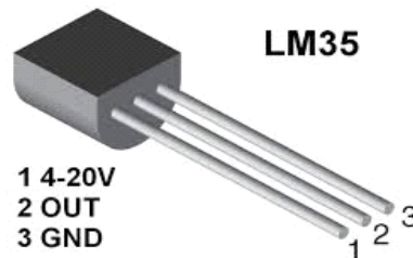
Fig(e).Temperature Sensor LM35
